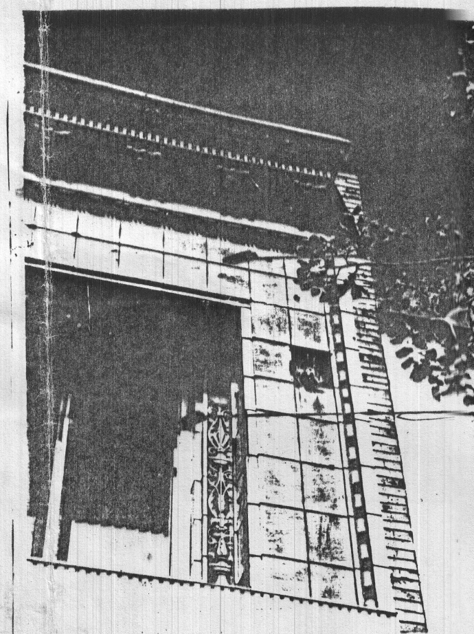
DETAIL PHOTO OF EXIST. ARCHITECTURAL TERRA-COTTA DETAIL
