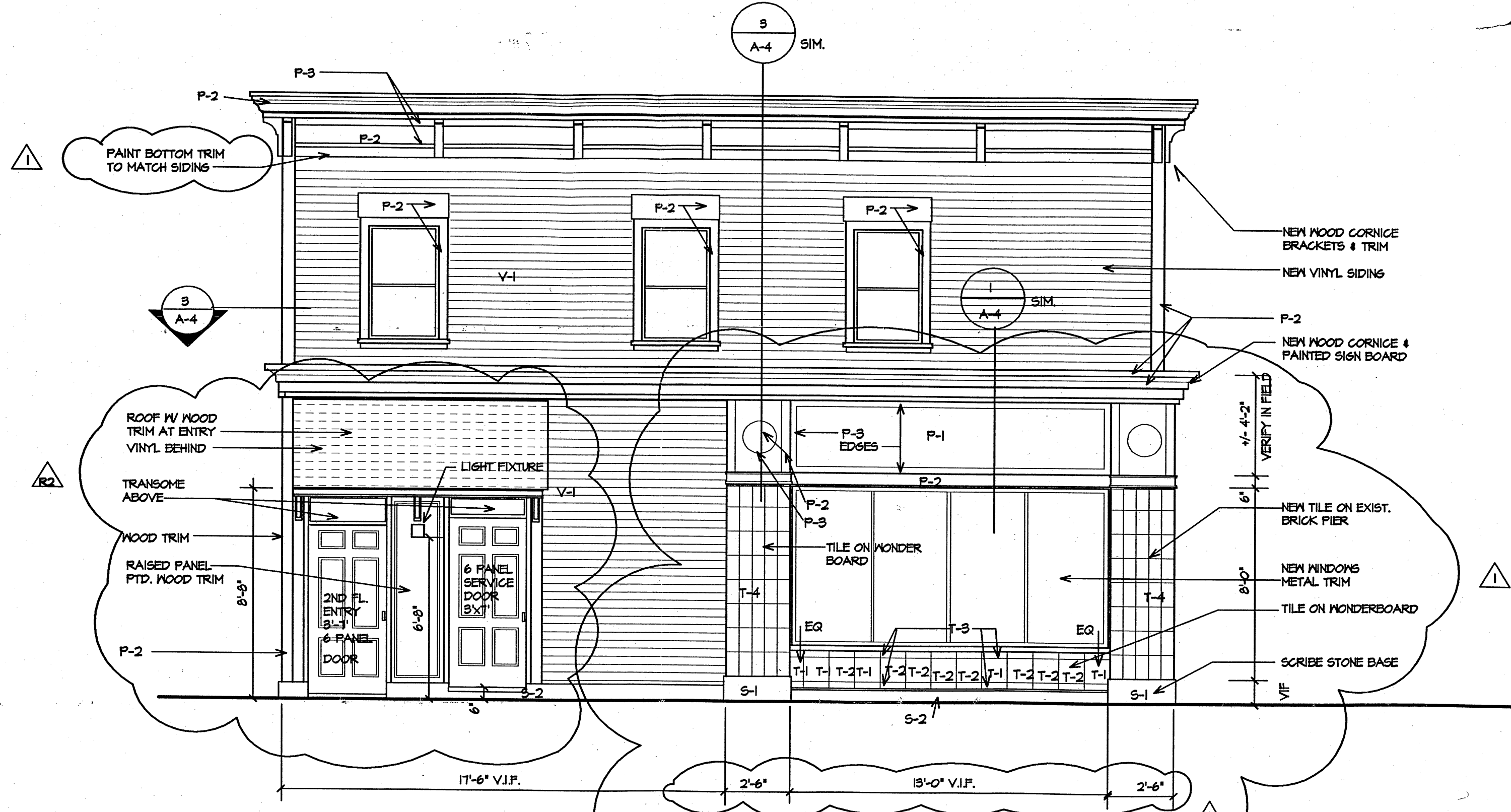
2 AMORY STREET ELEVATION A3 1/4" = 1'-0"
