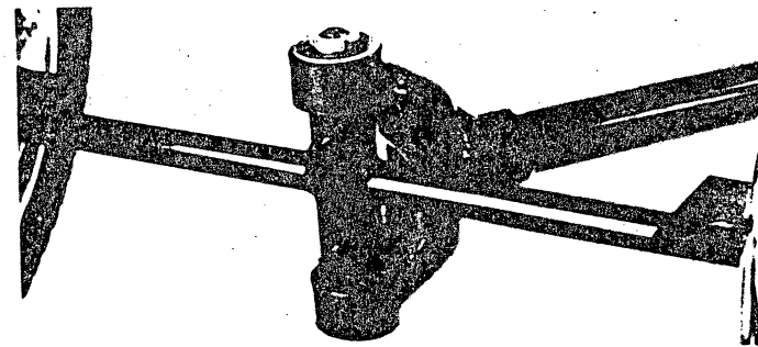
Machined Steering Spindle Cast Fitting. 1" Solid Steel Axle and Cross Lug
